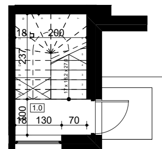
PARTER
